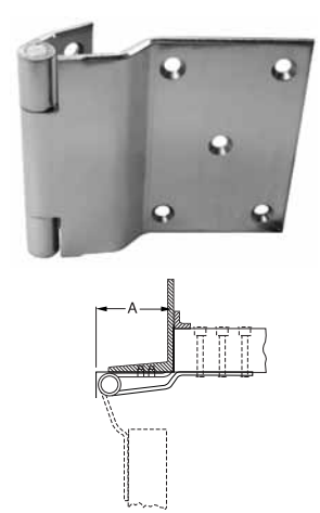
Full Surface CB1951R and STSCB1951R For channel iron frames
