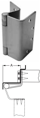
Full Mortise CB1948R and STSCB1948R {For square edge doors} (shown) CB1949R† and STSCB1949R† {For doors beveled 1/8" in 2" (3.2 in 51mm)}
